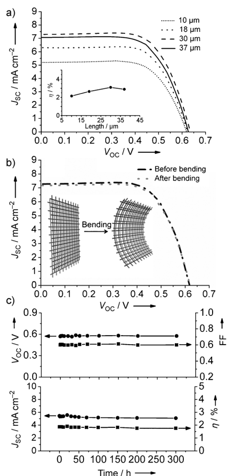
Figure 3. a) J – V curves of the DSC textile with an increase in the length of the \text{TiO}_2 nanotubes from 10 to 37 \mu\text{m} . Inset: Dependence of the energy conversion efficiency ( \eta ) on the length of the \text{TiO}_2 nanotubes. b) J – V curves of the DSC textile with a \text{TiO}_2 nanotube length of 30 \mu\text{m} before and after bending based on the liquid electrolyte. c) Time dependence of the photovoltaic parameters of the DSC textile that is based on the solid electrolyte.
