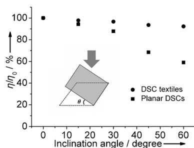
Figure 4. Dependence of the energy conversion efficiency on the incident light, measured by lifting one edge of a DSC textile with an angle of \theta . Here, \eta_0 and \eta correspond to the energy conversion efficiencies at 0° and at an angle of \theta , respectively.
